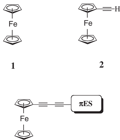
Diacetylene-group Connected Fc- \pi ES
