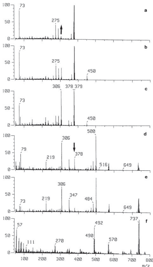
Figure 1. TMS removal of 5 (50 mg, 1.3 \times 10^{-1} mmol) with \text{K}_2\text{CO}_3 (1.3 mmol) in a mixture of MeOH and Py (1:1, 50 cm 3 ) was followed by MS measurements in a region of m/z 50–800. Each reaction mixture was quenched and treated similarly to the general reaction before measurement (see Experimental). MS spectra (a) after 15 min, (b) after 20 min, (c) after 30 min, (d) after 1 h, (e) after 2 h, and (f) the insoluble substances 4 .
